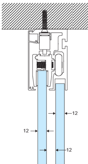
Ceiling Mounting
