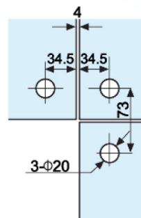
Connector for overpanel & sidepanel
