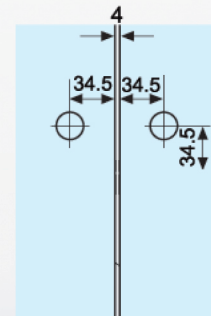
Connector for 2 glass panels
