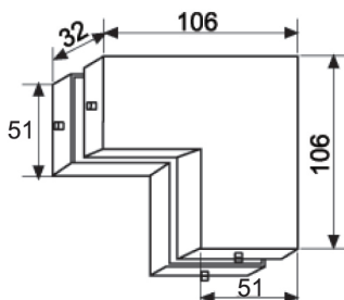
Connector for overpanel & sidepanel
