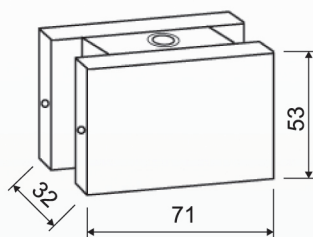
Side connector
