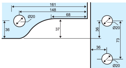
Overpanel to sidepanel pivot patch fitting
