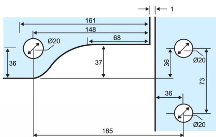
Overpanel to sidepanel pivot patch with fin fitting
